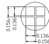
DOTS DETAIL (SCALE 10:1)
