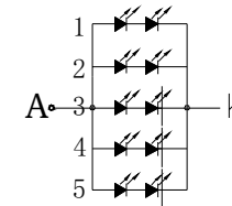
B/L CURCUIT DIAGRAM
