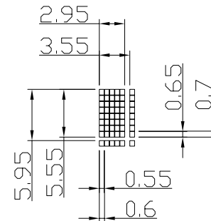
DISPLAY PATTERN
