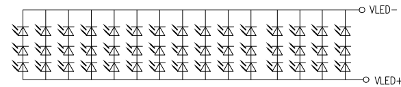
BACKLIGHT CIRCUIT DIAGRAM
