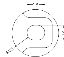
DETAIL B: SCALE 4:1
