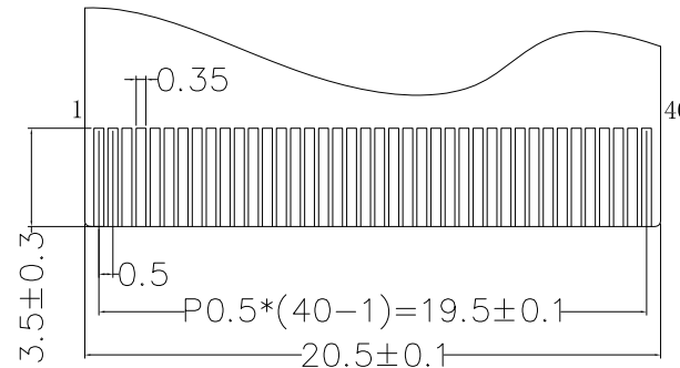
DETAIL A SCALE 5:1
