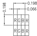
DETAIL A (SCALE 35:1)
