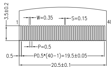
DETAIL B (SCALE 3:1)
