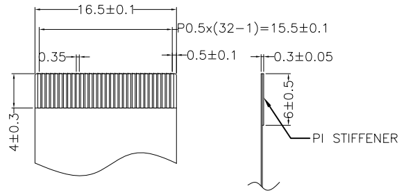
CN2 CONNECTOR MATED FPC/FFC STYLE (SCALE 2:1)
