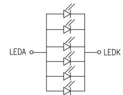
BACKLIGHT CIRCUIT DIAGRAM
