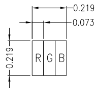
DETAIL A (SCALE 50:1)
