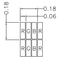
DETAIL A (SCALE 50:1)
