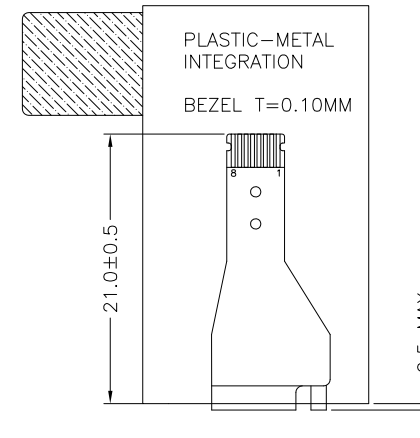
BENDING DIAGRAM FOR REFERENCE
