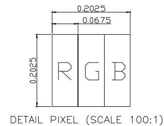
DETAIL PIXEL (SCALE 100:1)
