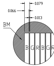
COLOR FILTER
