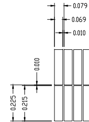
ITO DETAIL
