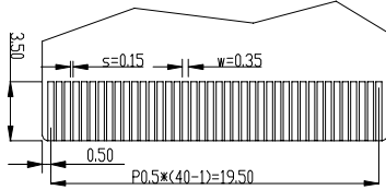
DETAIL A SCALE 4:1
