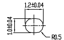
DETAIL B:
